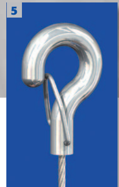
5 Wire hook with safety latch Opening gap 4 mm
