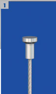
1 T-sleeve 2 Head Ø 6.0 mm Shaft Ø 3.5 mm Length 8.5 mm
